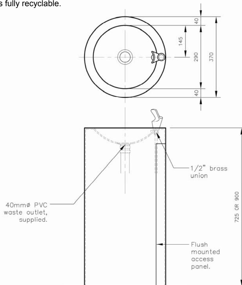
The Veitch Rondo drinking fountain comes complete with sturdy bubbler and PVC waste.
